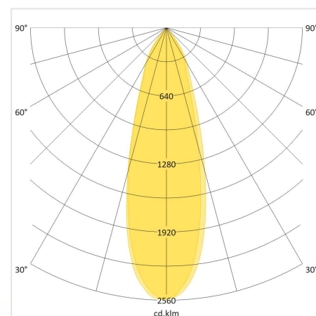
Flood 30°
