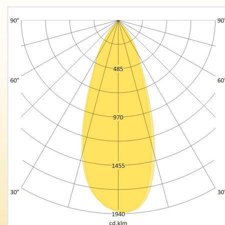
Wide Flood 40°
