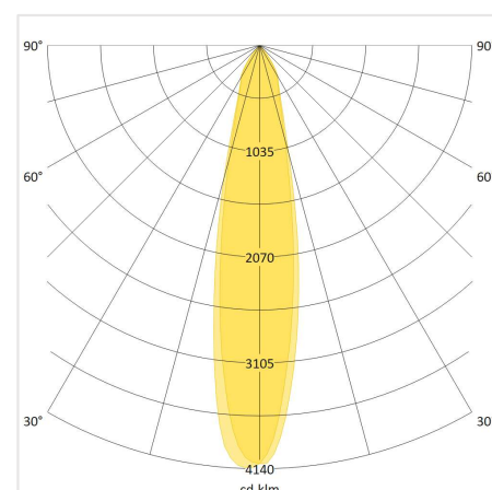
Narrow 20°
